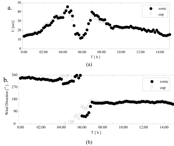
Fig. 2 10-min average wind speed and wind direction at height of 60m: (a) 10-min average wind speed and (b) 10-min average wind direction
