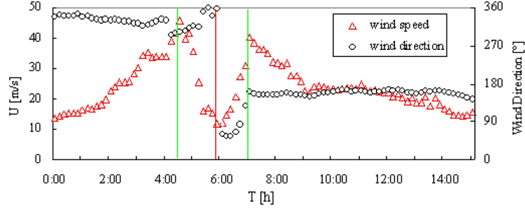
Fig. 3 10 min mean wind speed and direction of Typhoon Hagupit at 60 m height
