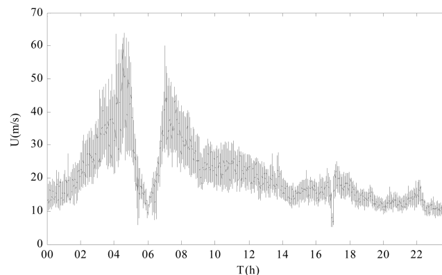
Fig. 4 Horizontal gust wind speed (0.1s) from the ultrasonic anemometer
