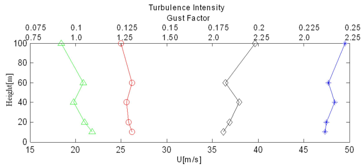
Fig. 10 Profiles of turbulence intensity, gust factor, mean wind speed and gust wind speed ( \diamond : 10 min mean wind speed, *: 3 s gust wind speed, \circ : gust factor, \triangle : turbulence intensity).
